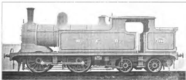
Fig. 5025. Eight-Wheel, Four-Coupled Tank Locomotive. North Eastern Railway. Cylinders 18 in. x 24 in.; Working Steam Pressure 160 lbs. per sq. in.; Total Heating Surface 1,697 sq. ft.; Weight on Drivers 67,440 lbs.; Total Weight 115,250 lbs.
